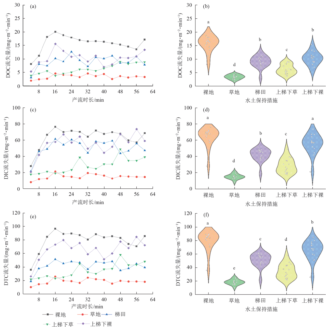
图 3 Changes in DOC , DIC and DTC loss volume under different soil and water conservation measures
